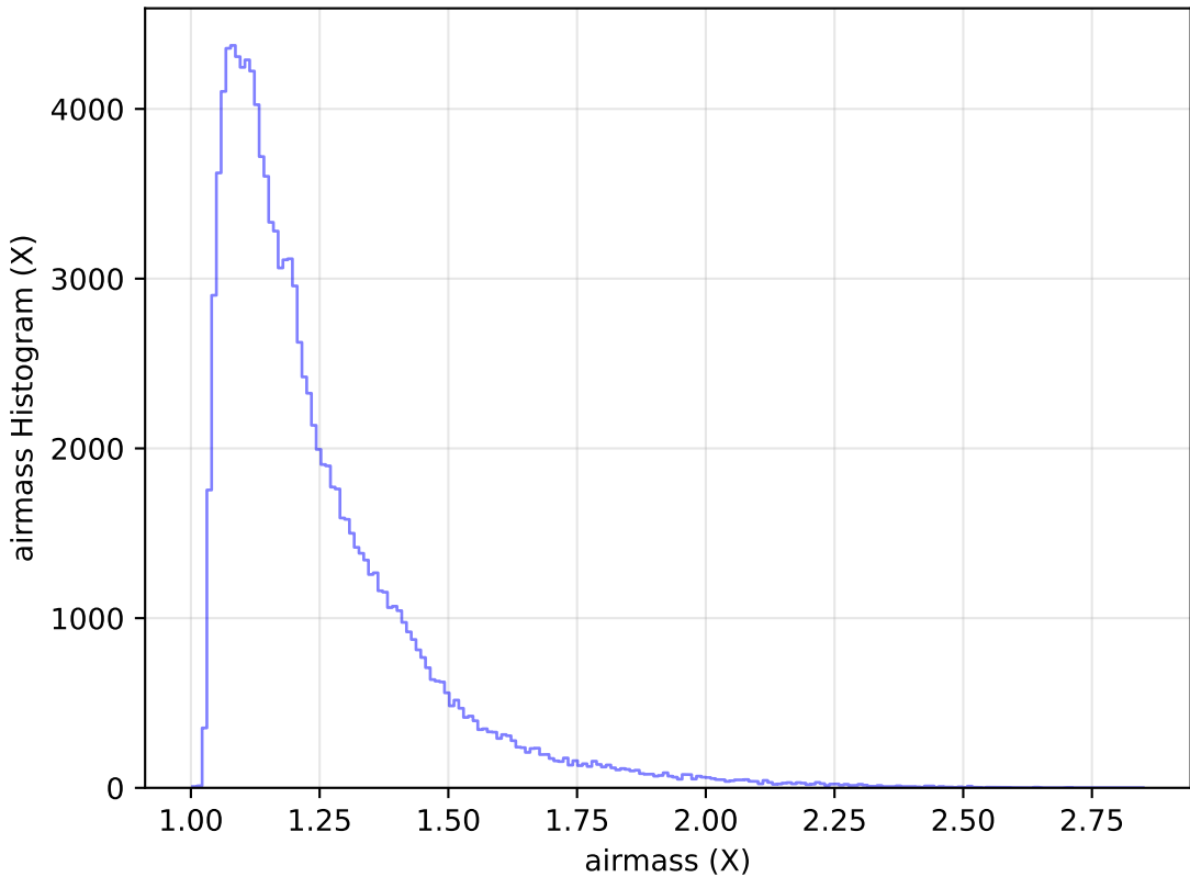
too_elab_r32_d2_giz_v3.4_10yrs WFD u band: airmass Histogram
