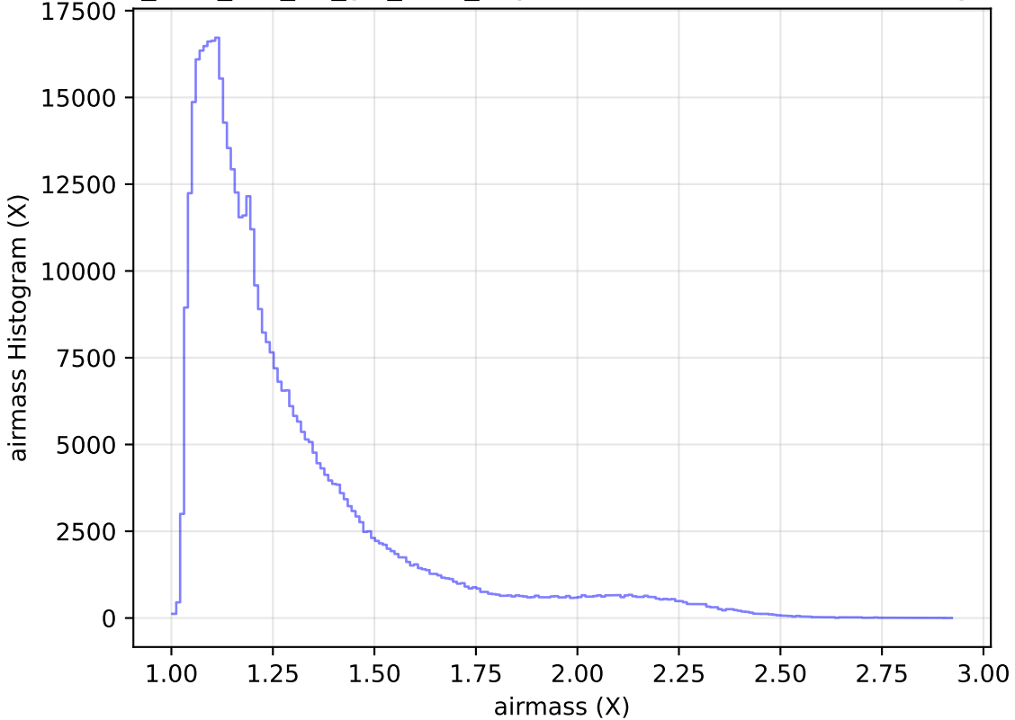
too_elab_r32_d2_giz_v3.4_10yrs WFD r band: airmass Histogram
