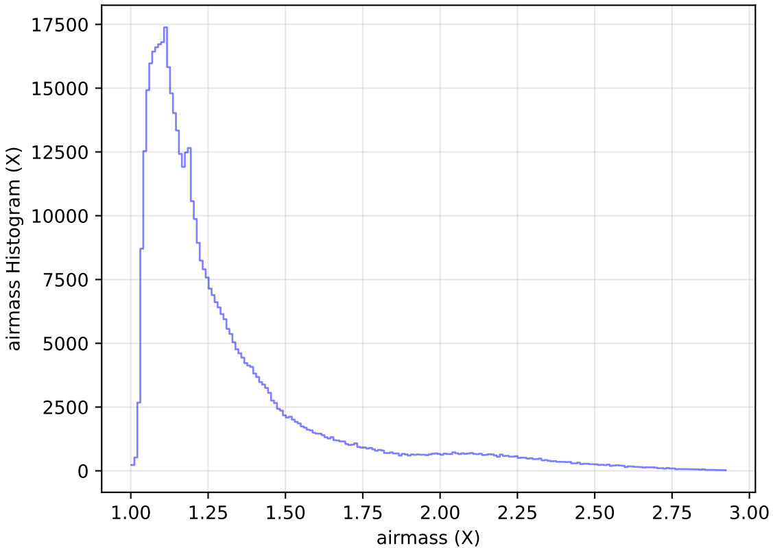
too_elab_r32_d2_giz_v3.4_10yrs WFD i band: airmass Histogram
