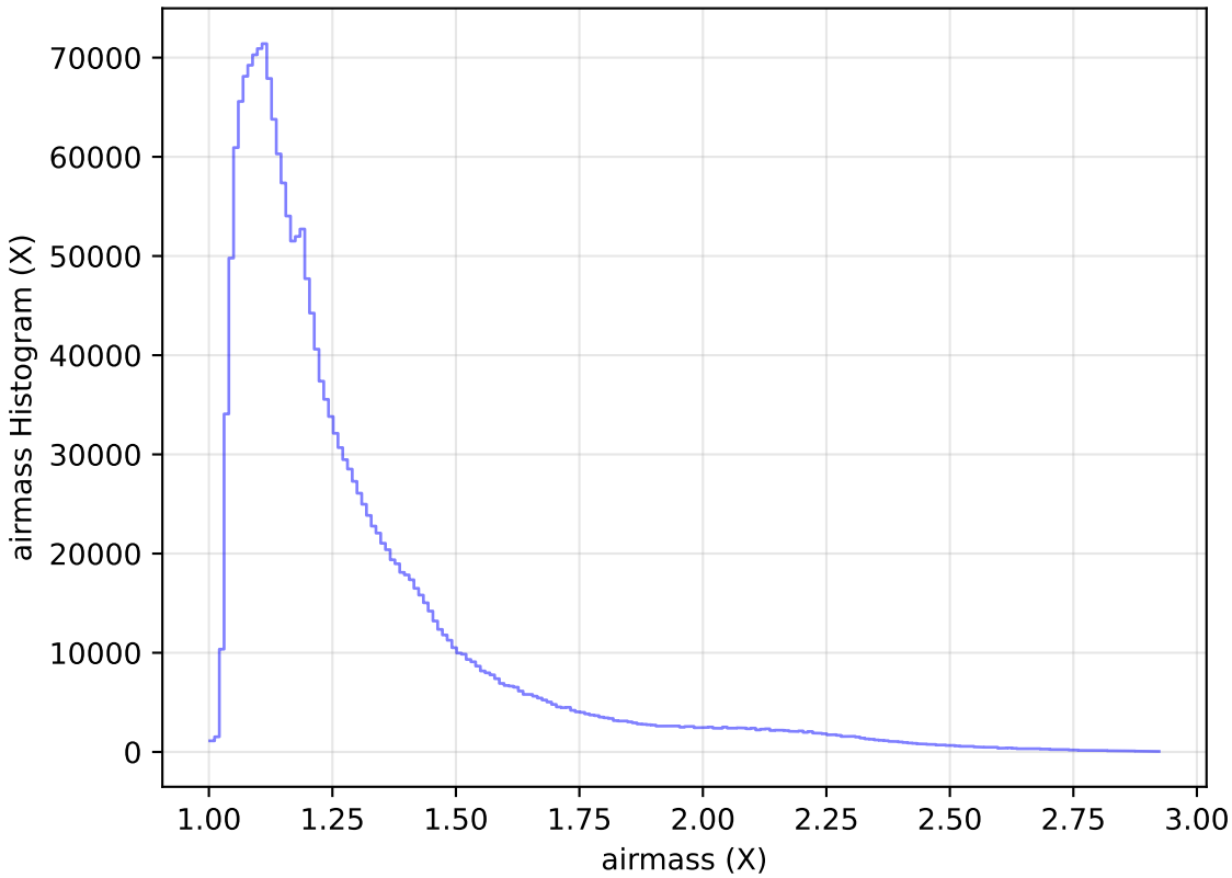
too_elab_r32_d2_giz_v3.4_10yrs WFD all bands: airmass Histogram
