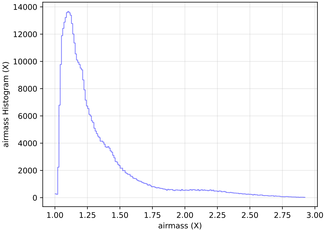
too_elab_r32_d2_giz_v3.4_10yrs All sky z band: airmass Histogram
