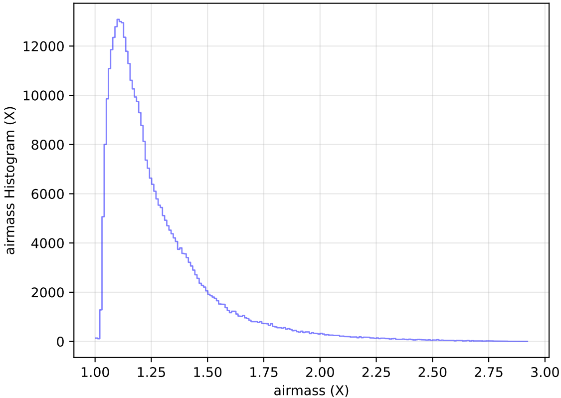
too_elab_r32_d2_giz_v3.4_10yrs All sky y band: airmass Histogram
