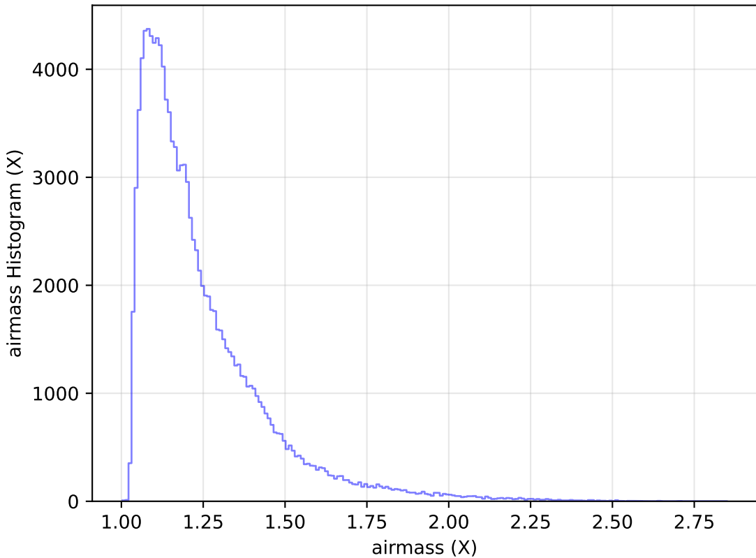
too_elab_r32_d2_giz_v3.4_10yrs All sky u band: airmass Histogram
