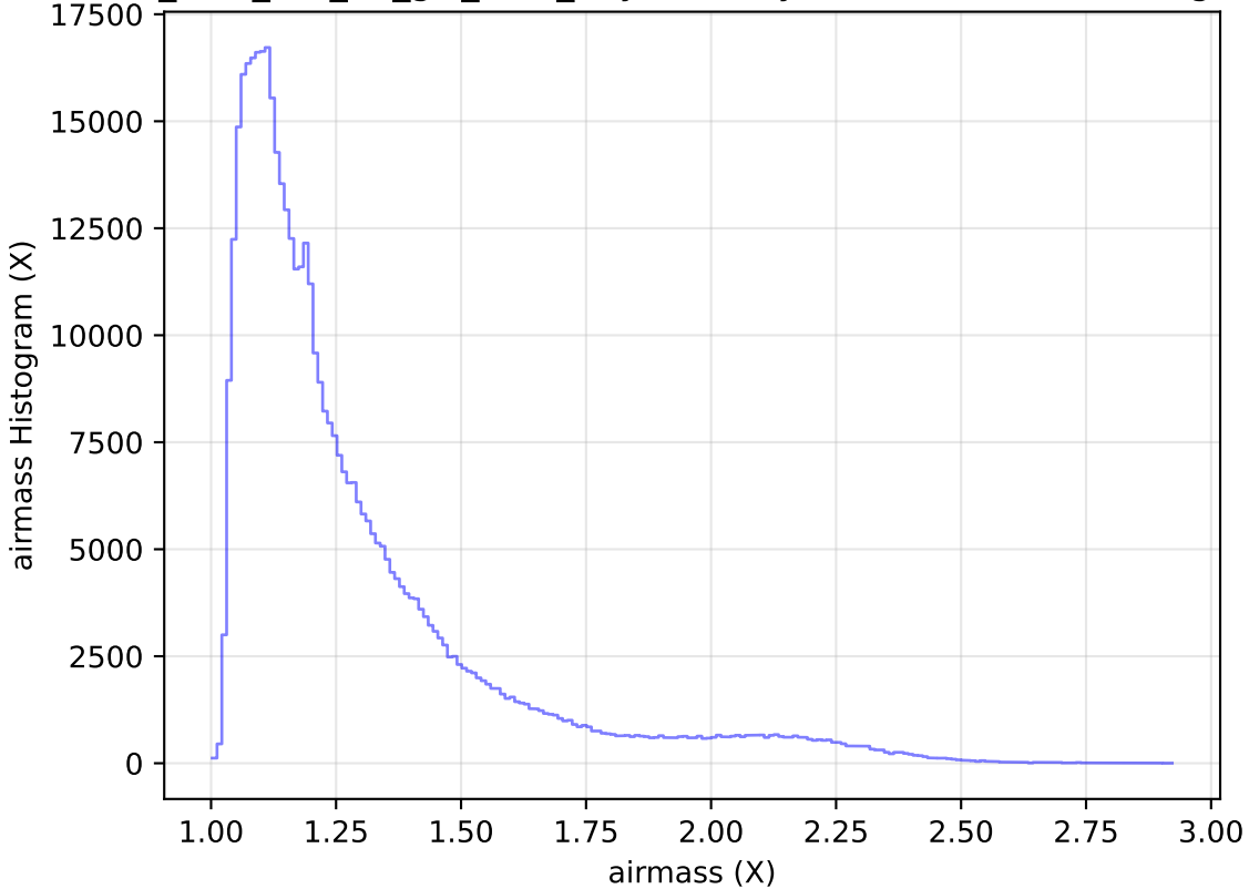
too_elab_r32_d2_giz_v3.4_10yrs All sky r band: airmass Histogram
