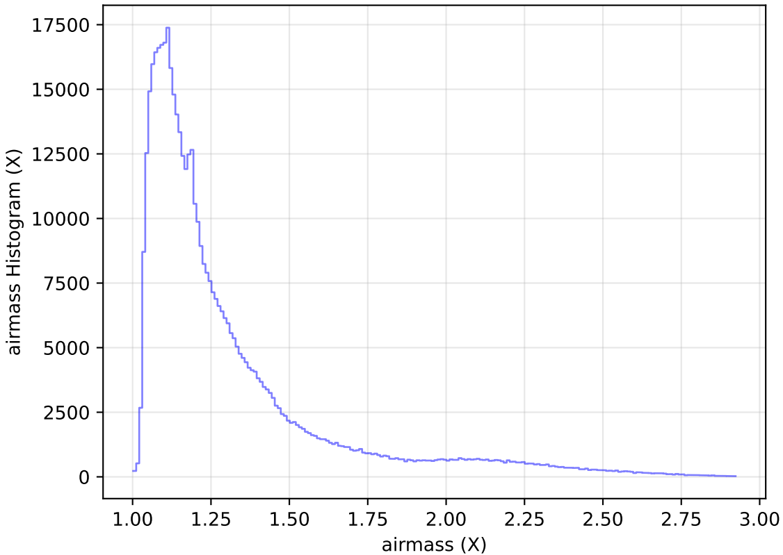
too_elab_r32_d2_giz_v3.4_10yrs All sky i band: airmass Histogram
