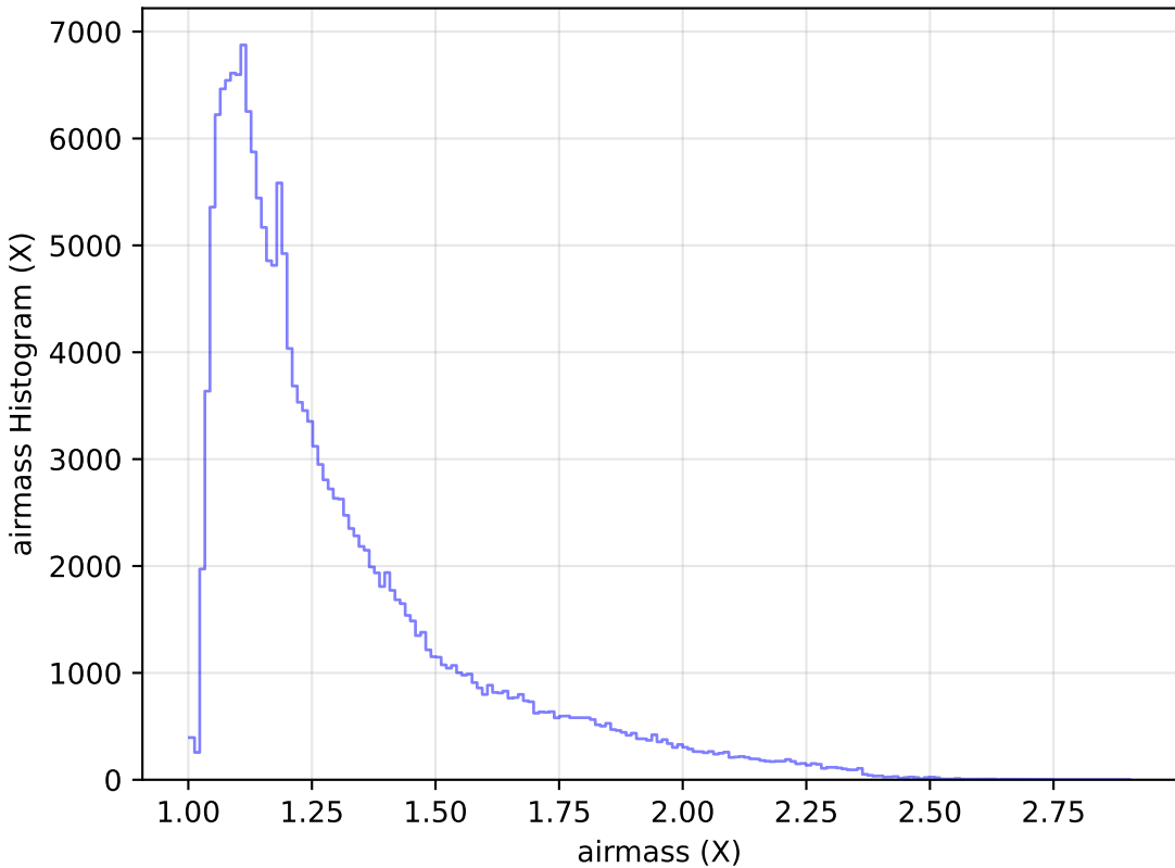
too_elab_r32_d2_giz_v3.4_10yrs All sky g band: airmass Histogram
