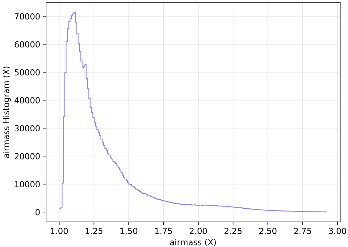
too_elab_r32_d2_giz_v3.4_10yrs All sky all bands: airmass Histogram
