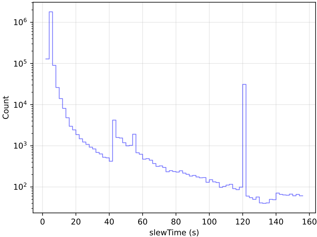
too_elab_r32_d2_giz_v3.4_10yrs All visits: Slew Time Histogram
