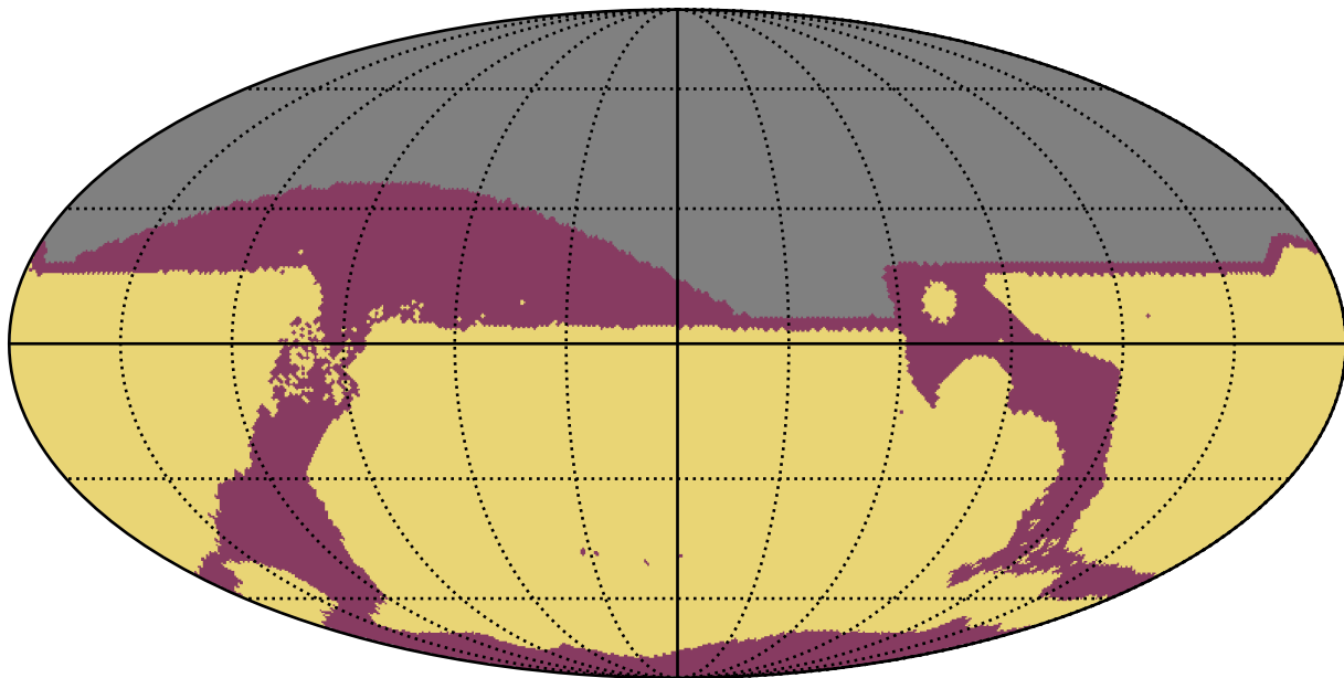
too_elab_r32_d2_giz_v3.4_10yrs All sky: RapidRevisits
