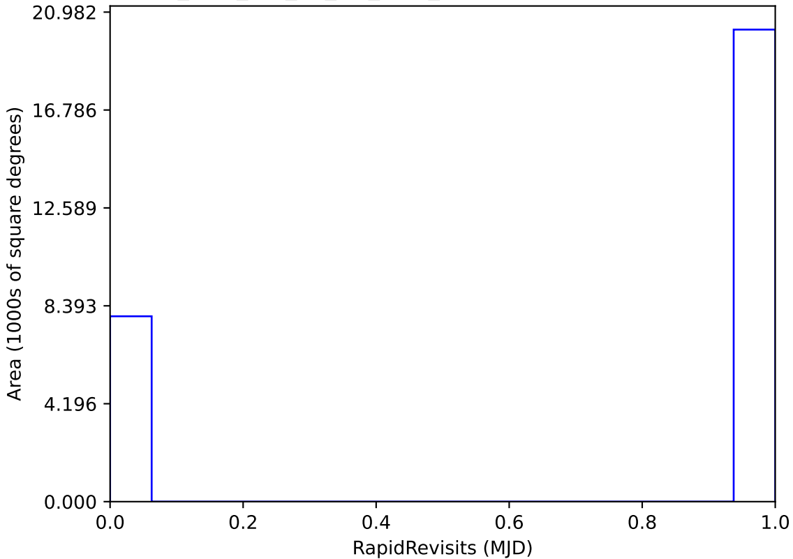
too_elab_r32_d2_giz_v3.4_10yrs All sky: RapidRevisits
