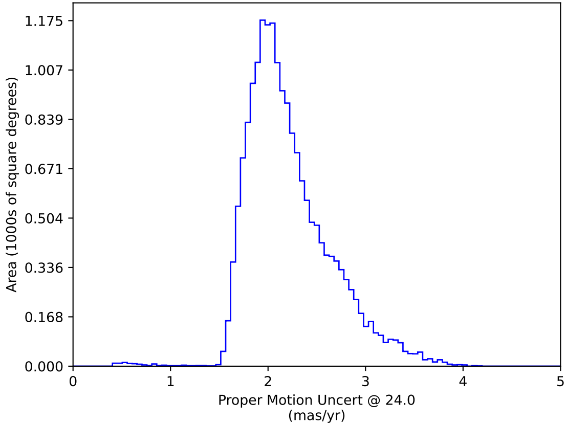
too_elab_r32_d2_giz_v3.4_10yrs WFD: Proper Motion Uncert @ 24.0
