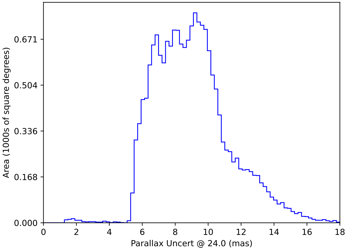
too_elab_r32_d2_giz_v3.4_10yrs WFD: Parallax Uncert @ 24.0
