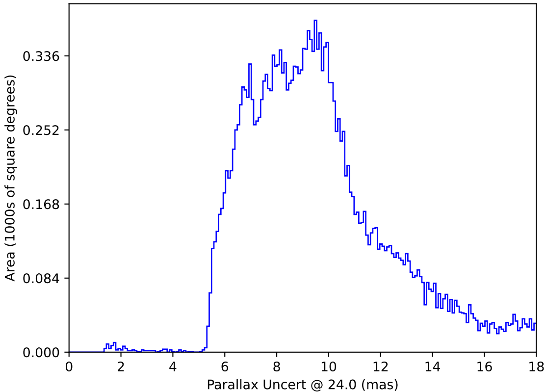
too_elab_r32_d2_giz_v3.4_10yrs All sky: Parallax Uncert @ 24.0
