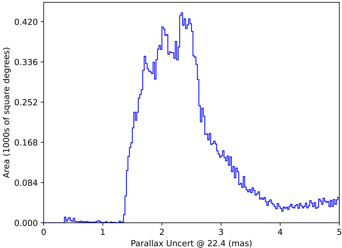
too_elab_r32_d2_giz_v3.4_10yrs All sky: Parallax Uncert @ 22.4
