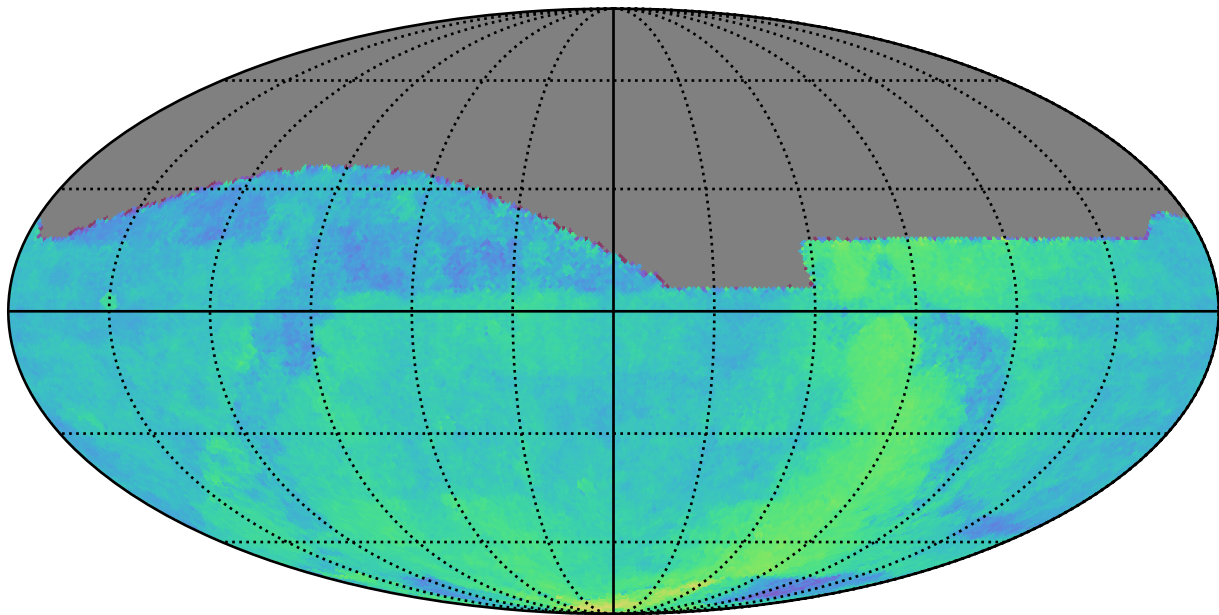
too_elab_r32_d2_giz_v3.4_10yrs All sky: Parallax Coverage @ 24.0
