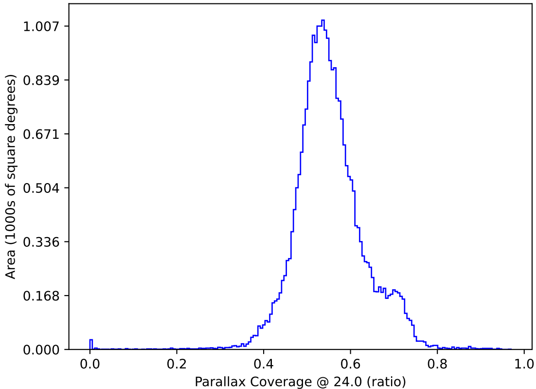
too_elab_r32_d2_giz_v3.4_10yrs All sky: Parallax Coverage @ 24.0
