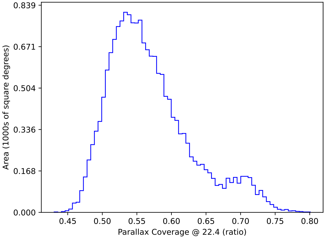
too_elab_r32_d2_giz_v3.4_10yrs WFD: Parallax Coverage @ 22.4
