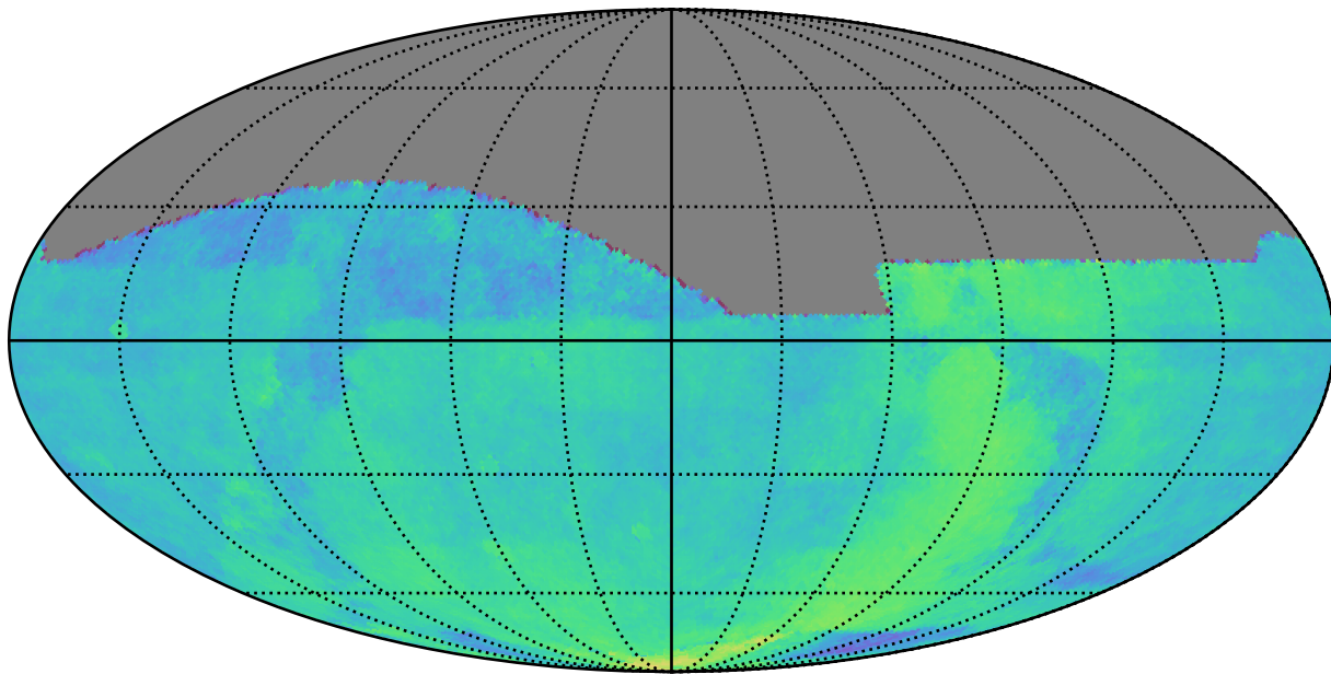
too_elab_r32_d2_giz_v3.4_10yrs All sky: Parallax Coverage @ 22.4
