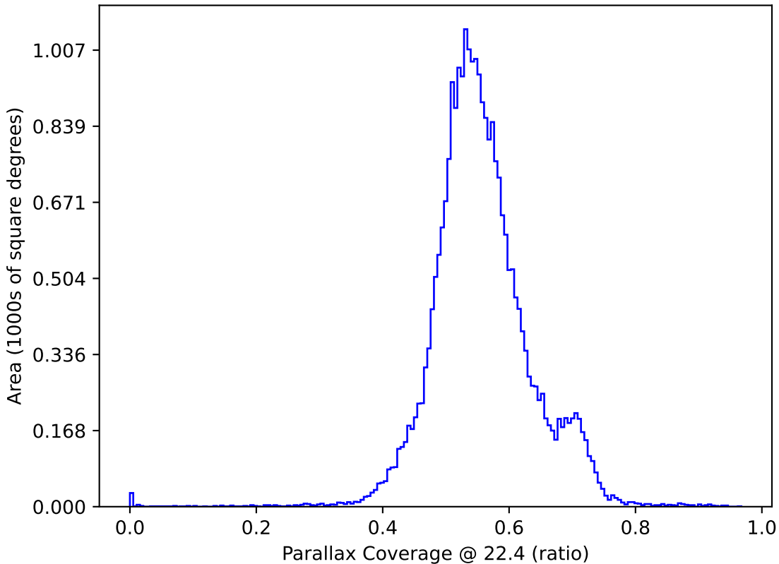
too_elab_r32_d2_giz_v3.4_10yrs All sky: Parallax Coverage @ 22.4
