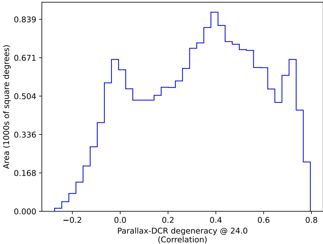
too_elab_r32_d2_giz_v3.4_10yrs WFD: Parallax-DCR degeneracy @ 24.0
