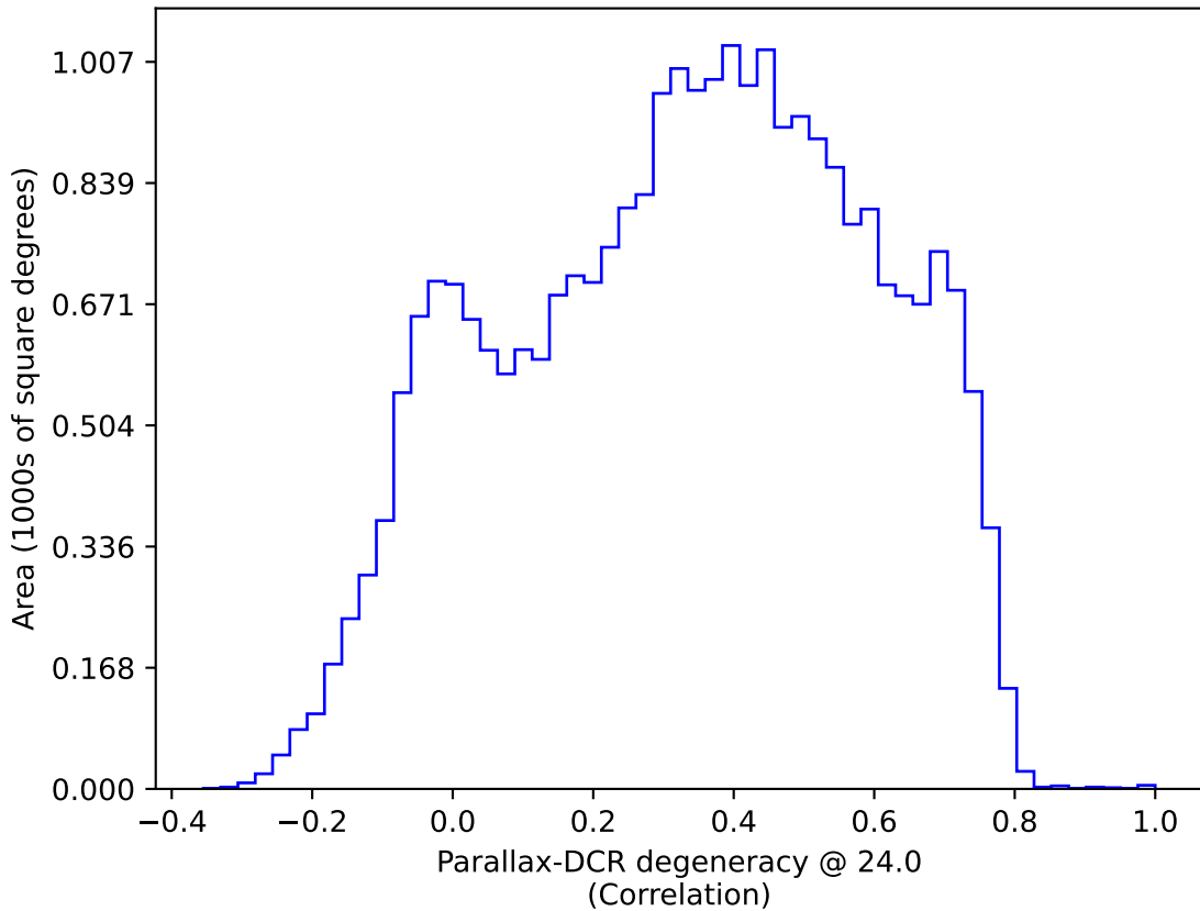
too_elab_r32_d2_giz_v3.4_10yrs All sky: Parallax-DCR degeneracy @ 24.0
