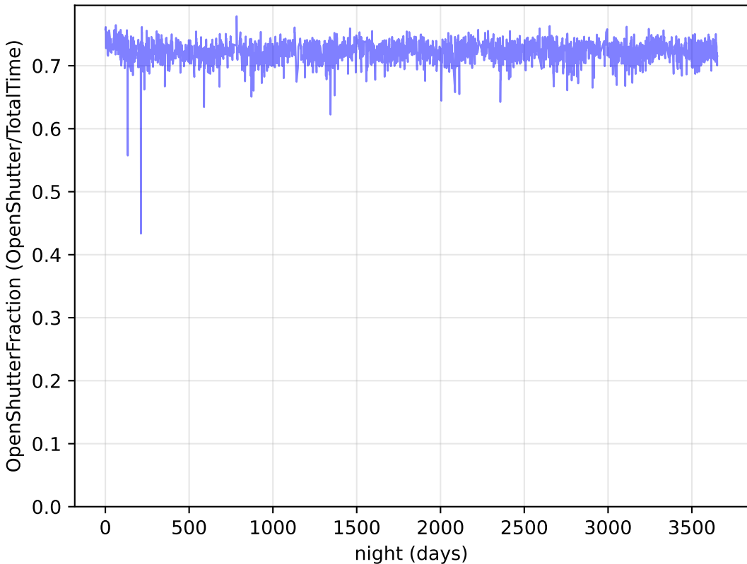
too_elab_r32_d2_giz_v3.4_10yrs Per night: OpenShutterFraction
