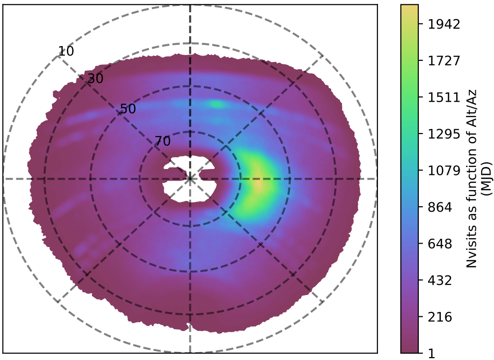
too_elab_r32_d2_giz_v3.4_10yrs y band: Nvisits as function of Alt/Az
