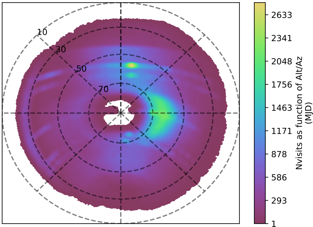
too_elab_r32_d2_giz_v3.4_10yrs r band: Nvisits as function of Alt/Az
