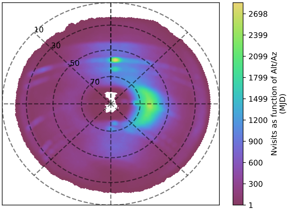
too_elab_r32_d2_giz_v3.4_10yrs i band: Nvisits as function of Alt/Az
