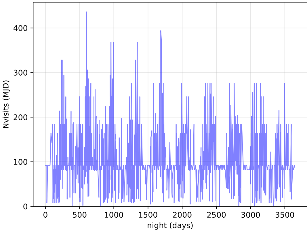
too_elab_r32_d2_giz_v3.4_10yrs DDF: Nvisits
