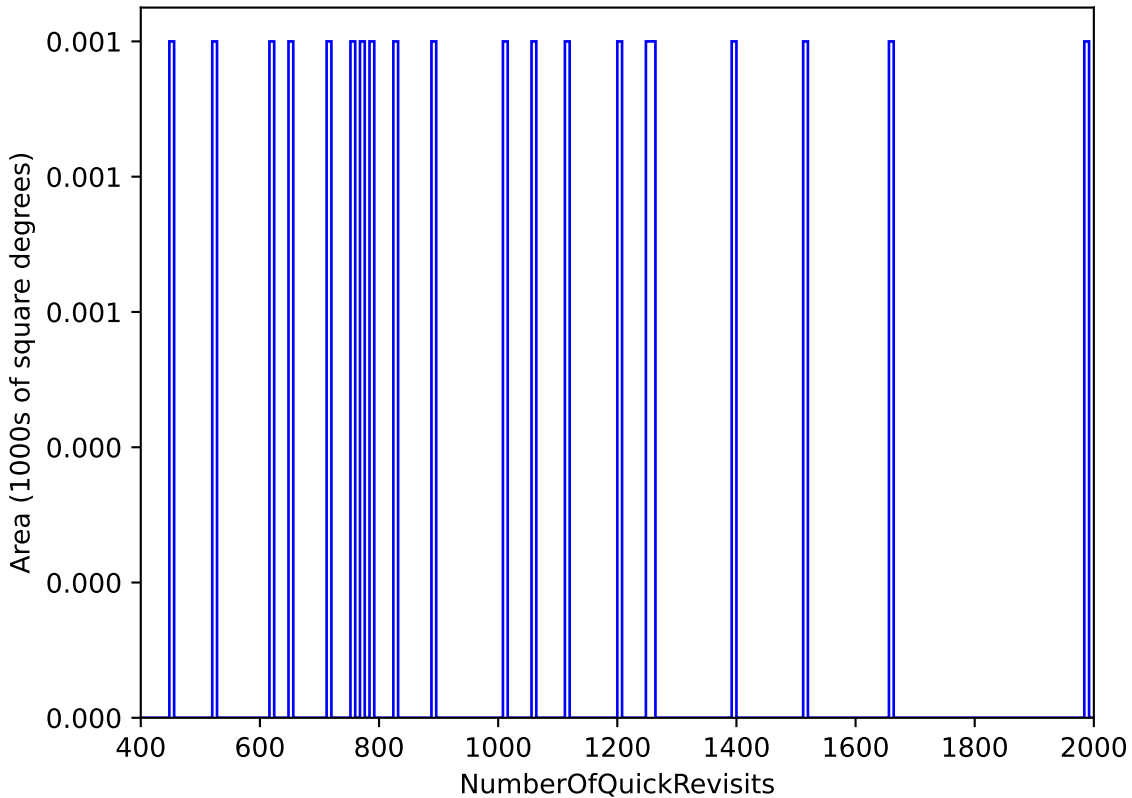
too_elab_r32_d2_giz_v3.4_10yrs WFD: NumberOfQuickRevisits
