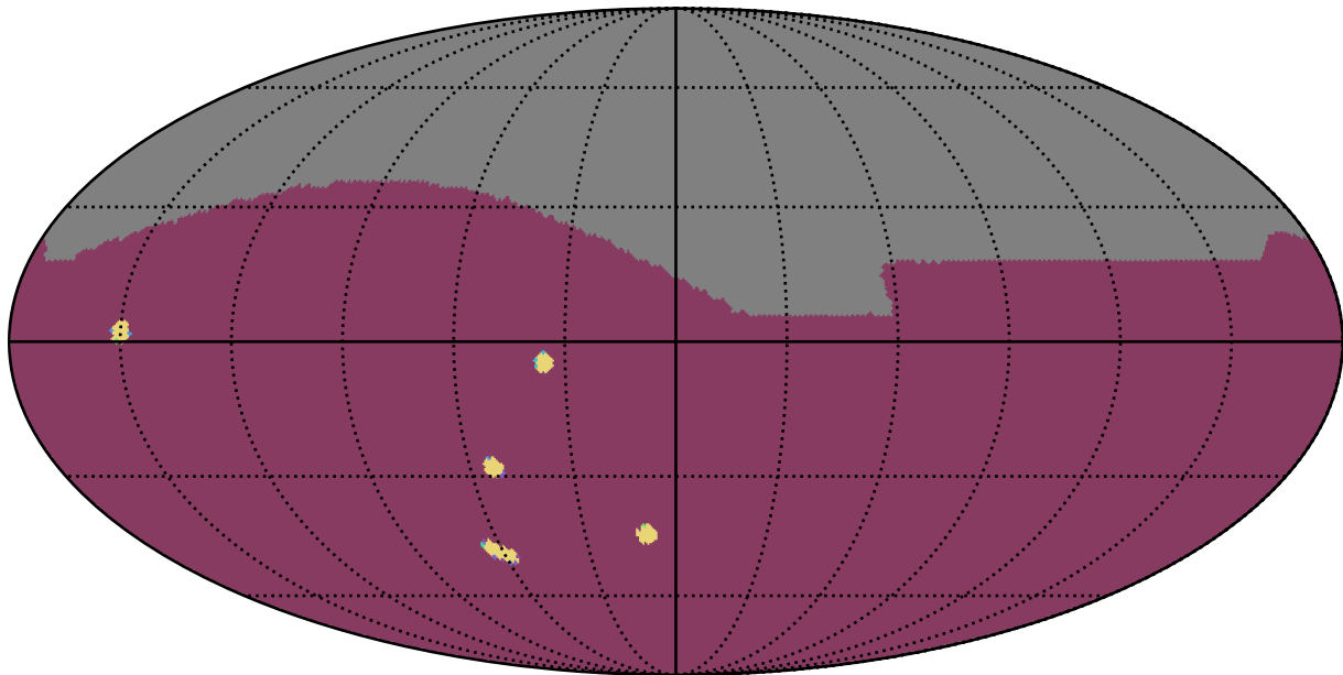
too_elab_r32_d2_giz_v3.4_10yrs All sky: NumberOfQuickRevisits
