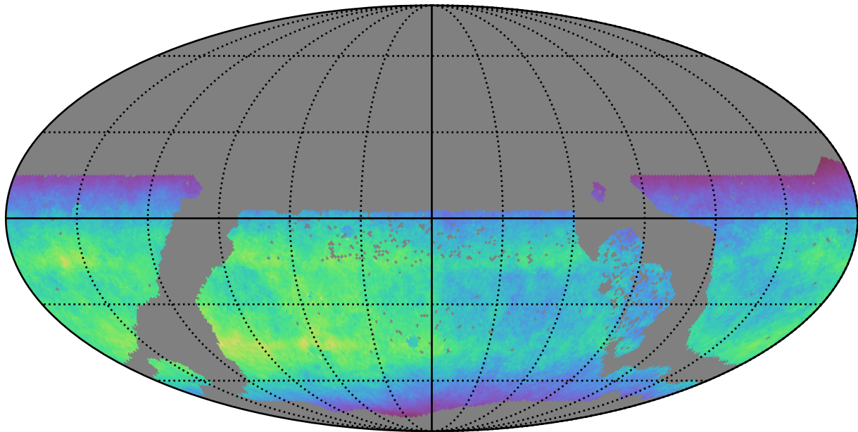
too_elab_r32_d2_giz_v3.4_10yrs WFD y band: Normalized Teff
