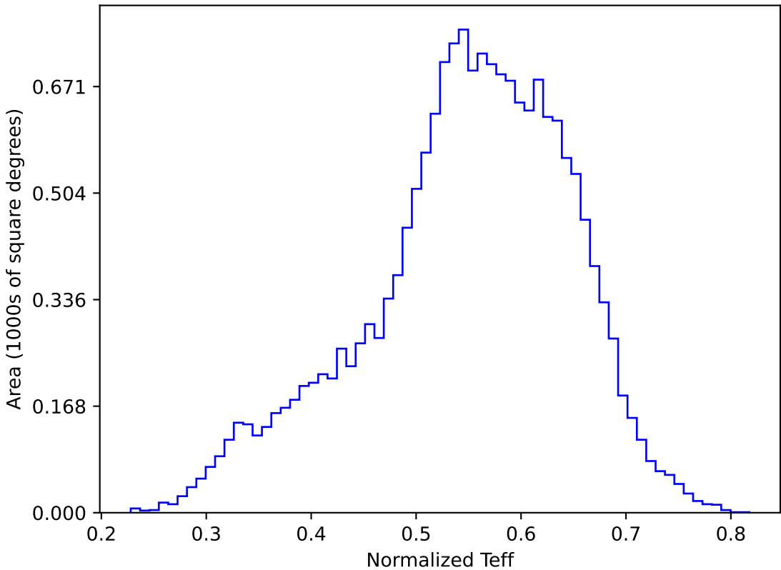
too_elab_r32_d2_giz_v3.4_10yrs WFD y band: Normalized Teff
