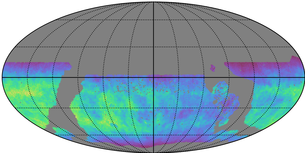
too_elab_r32_d2_giz_v3.4_10yrs WFD u band: Normalized Teff
