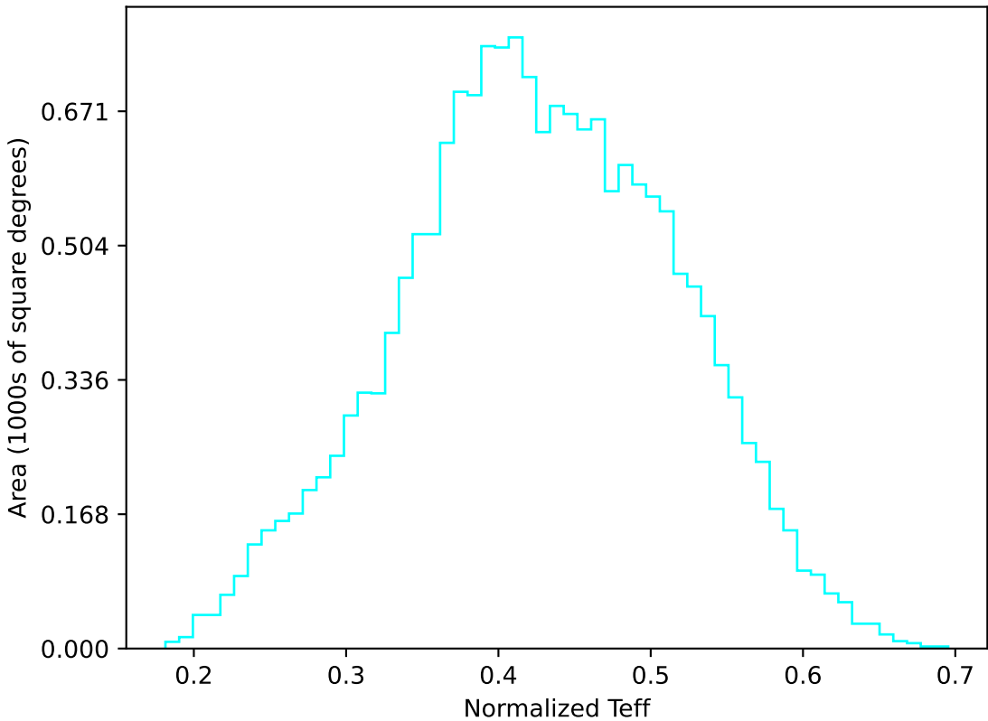
too_elab_r32_d2_giz_v3.4_10yrs WFD u band: Normalized Teff
