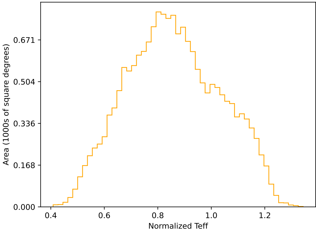
too_elab_r32_d2_giz_v3.4_10yrs WFD r band: Normalized Teff
