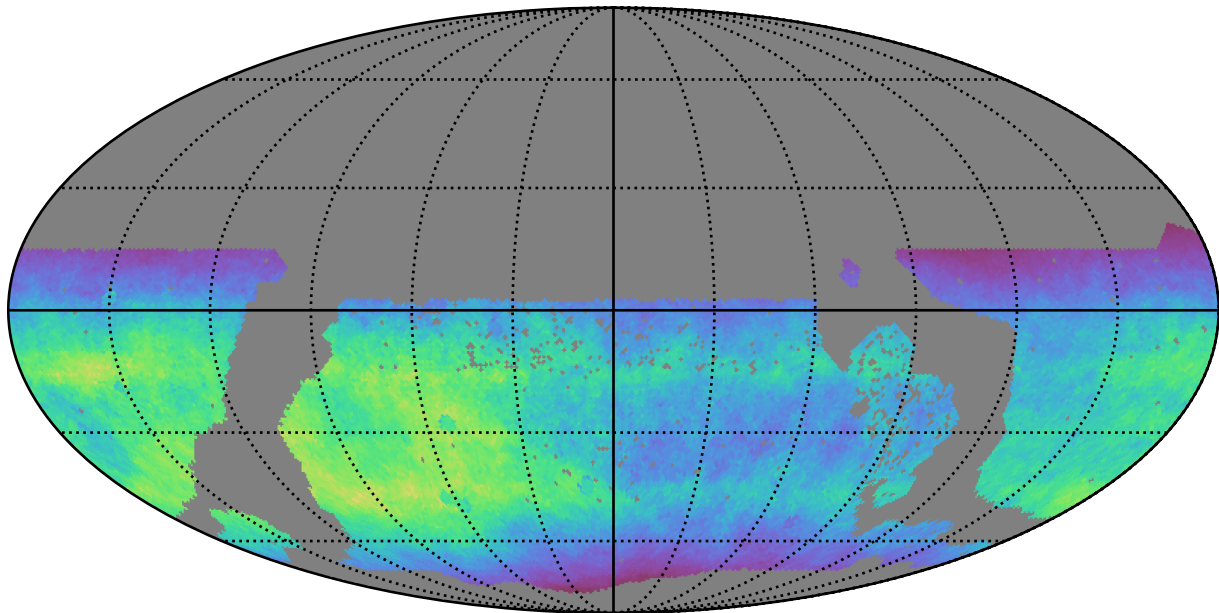
too_elab_r32_d2_giz_v3.4_10yrs WFD i band: Normalized Teff
