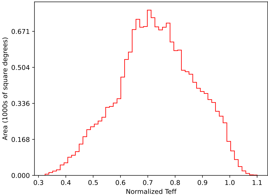
too_elab_r32_d2_giz_v3.4_10yrs WFD i band: Normalized Teff
