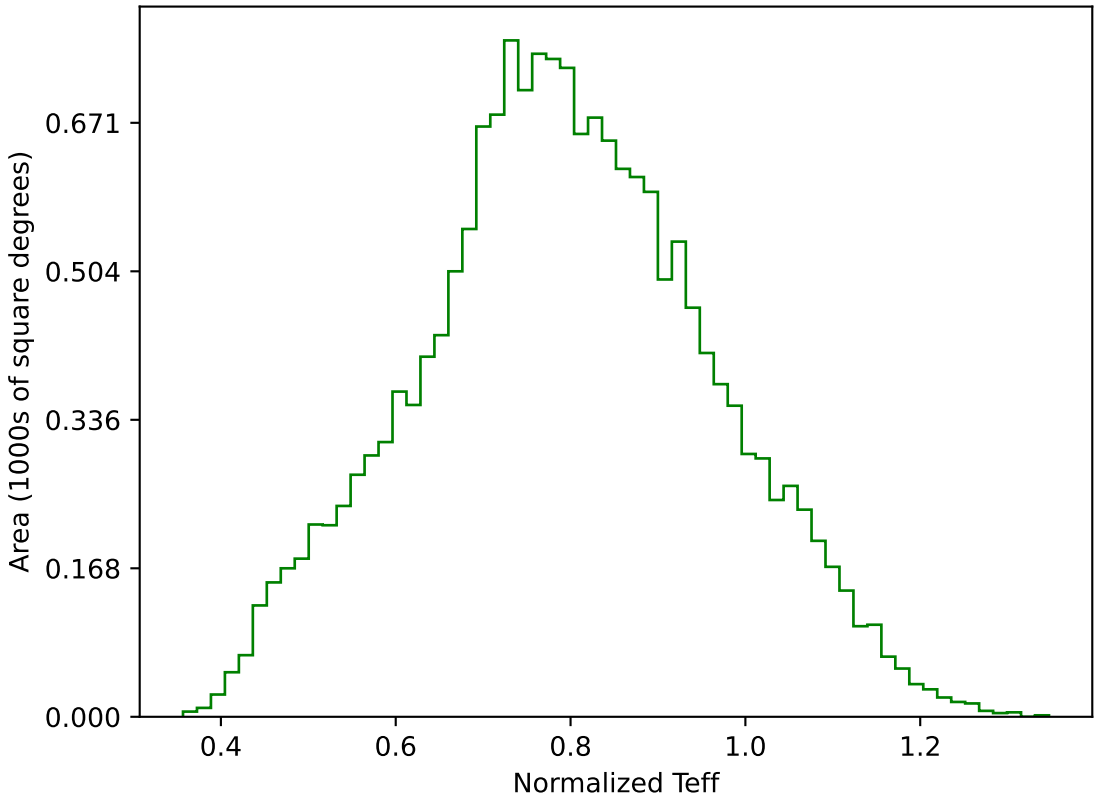
too_elab_r32_d2_giz_v3.4_10yrs WFD g band: Normalized Teff
