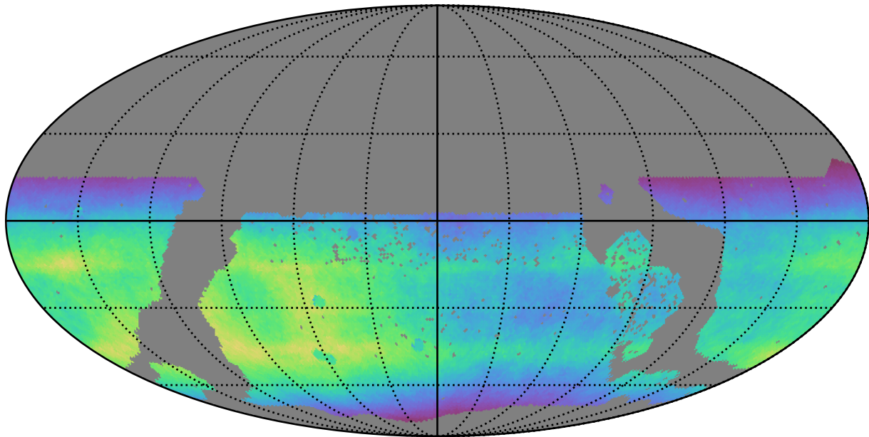
too_elab_r32_d2_giz_v3.4_10yrs WFD all bands: Normalized Teff
