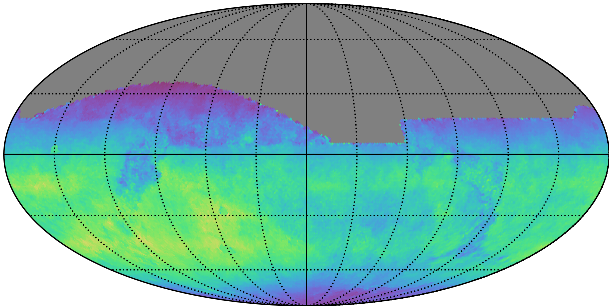
too_elab_r32_d2_giz_v3.4_10yrs All sky z band: Normalized Teff
