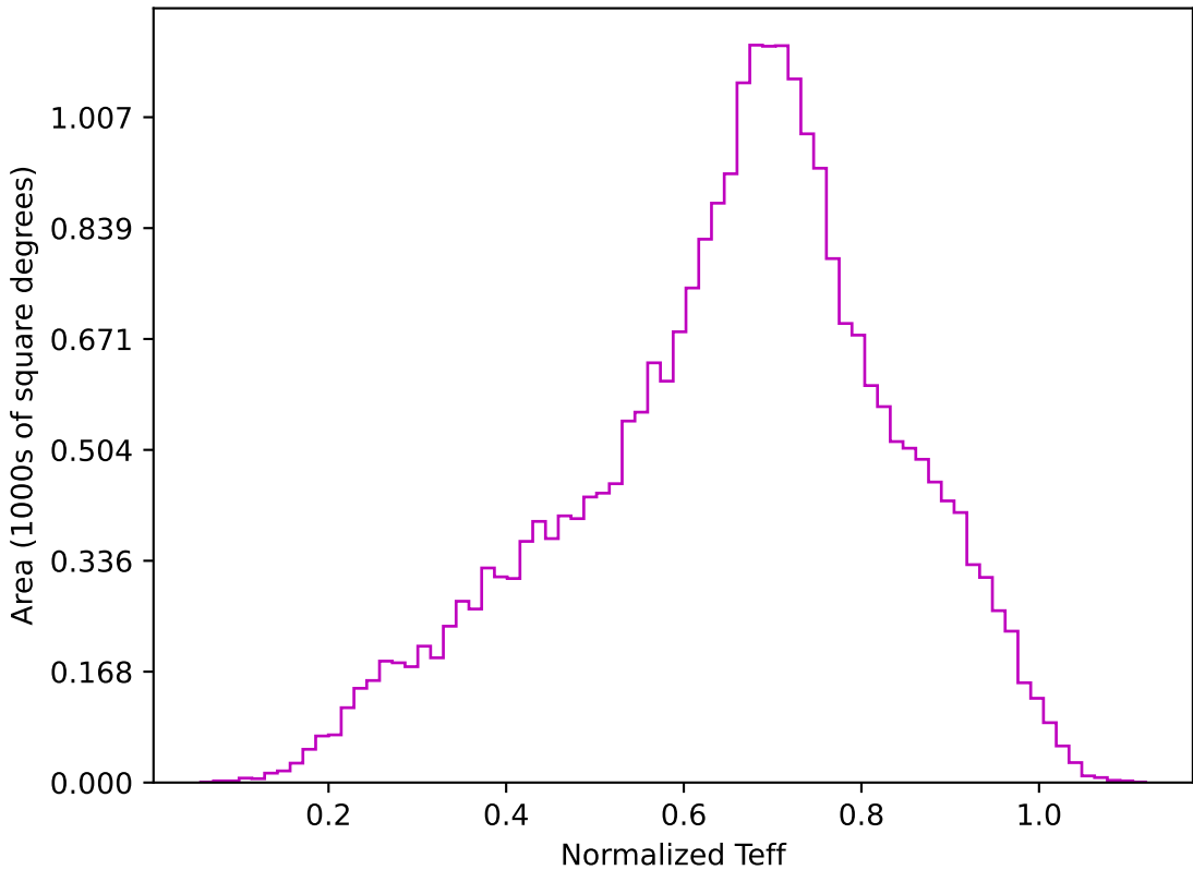
too_elab_r32_d2_giz_v3.4_10yrs All sky z band: Normalized Teff
