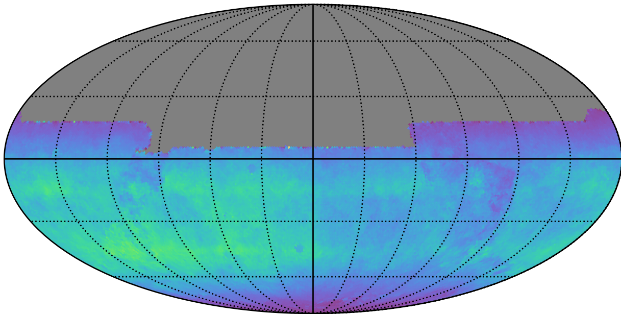
too_elab_r32_d2_giz_v3.4_10yrs All sky y band: Normalized Teff
