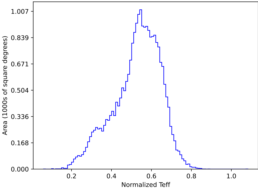
too_elab_r32_d2_giz_v3.4_10yrs All sky y band: Normalized Teff
