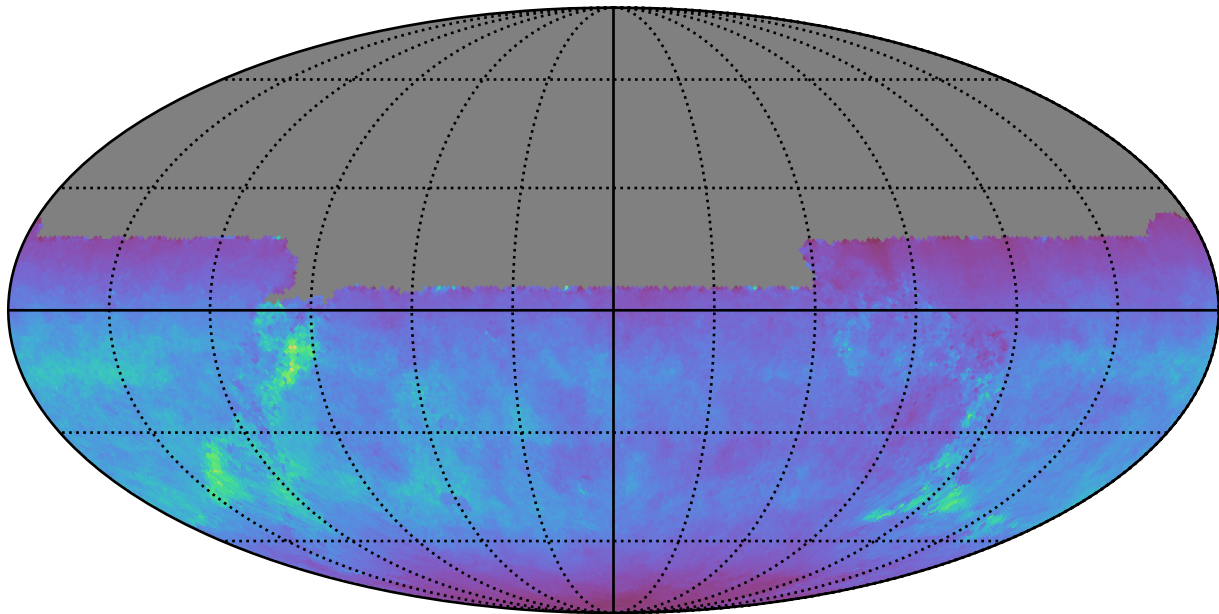
too_elab_r32_d2_giz_v3.4_10yrs All sky u band: Normalized Teff
