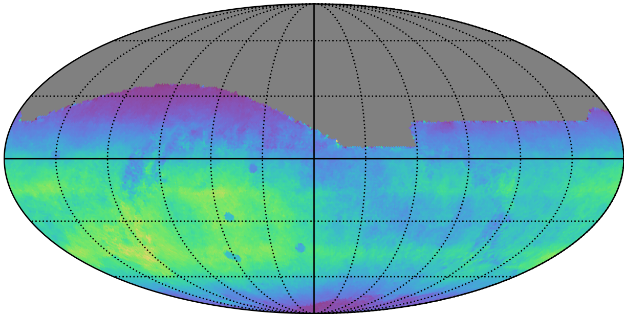
too_elab_r32_d2_giz_v3.4_10yrs All sky r band: Normalized Teff
