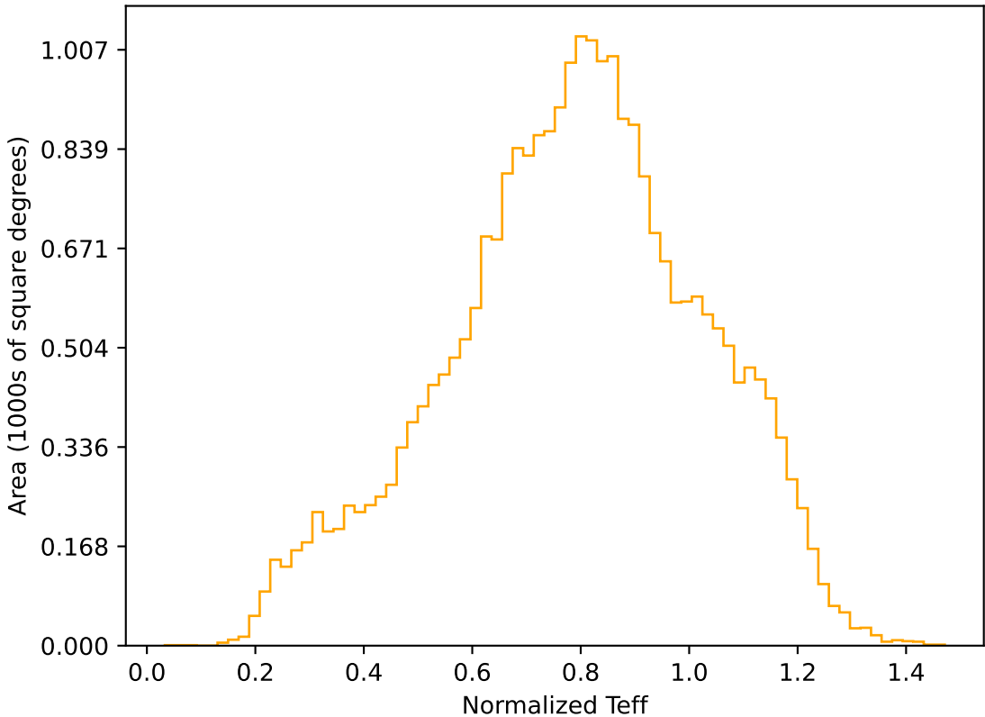
too_elab_r32_d2_giz_v3.4_10yrs All sky r band: Normalized Teff
