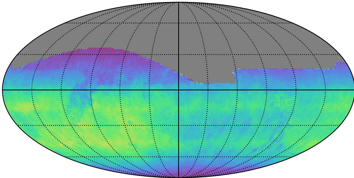
too_elab_r32_d2_giz_v3.4_10yrs All sky i band: Normalized Teff
