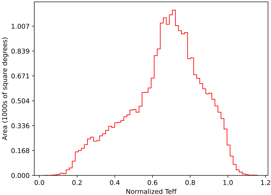
too_elab_r32_d2_giz_v3.4_10yrs All sky i band: Normalized Teff
